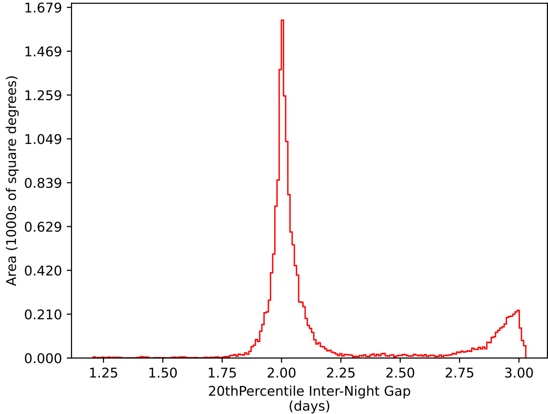
ddf_acor_sf20_lsf40_lsr10_v3.4_10yrs WFD i band: 20thPercentile Inter-Night Gap
