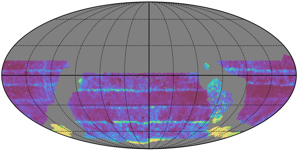
ddf_acor_sf20_lsf40_lsr10_v3.4_10yrs WFD all bands: 20thPercentile Inter-Night Gap
