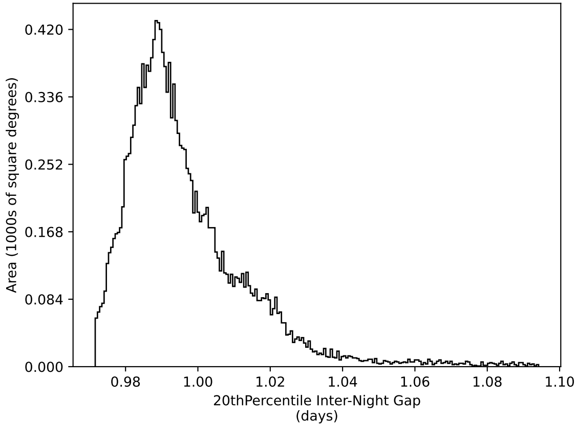
ddf_acor_sf20_lsf40_lsr10_v3.4_10yrs WFD all bands: 20thPercentile Inter-Night Gap
