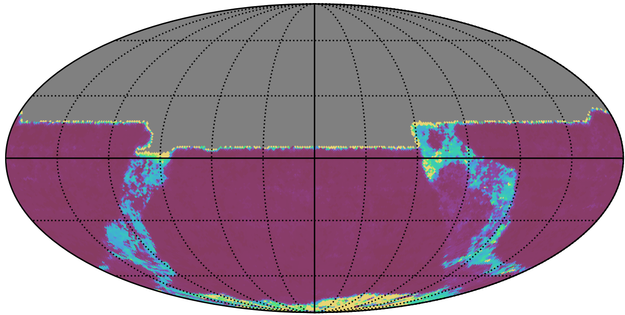
ddf_acor_sf20_lsf40_lsr10_v3.4_10yrs All sky y band: 20thPercentile Inter-Night Gap
