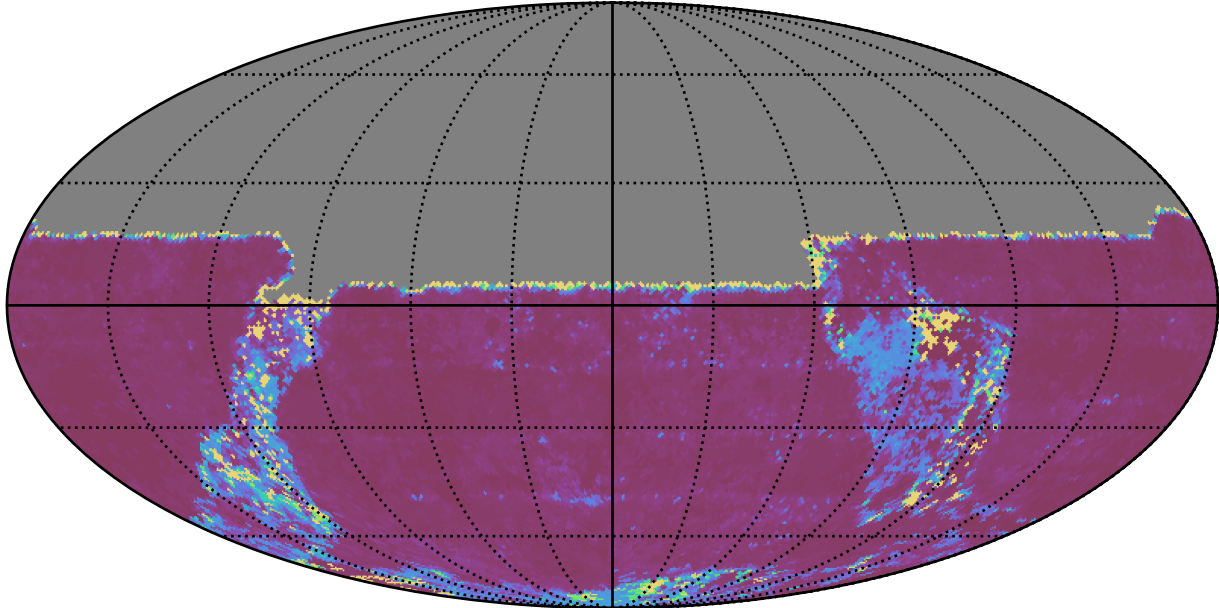
ddf_acor_sf20_lsf40_lsr10_v3.4_10yrs All sky u band: 20thPercentile Inter-Night Gap
