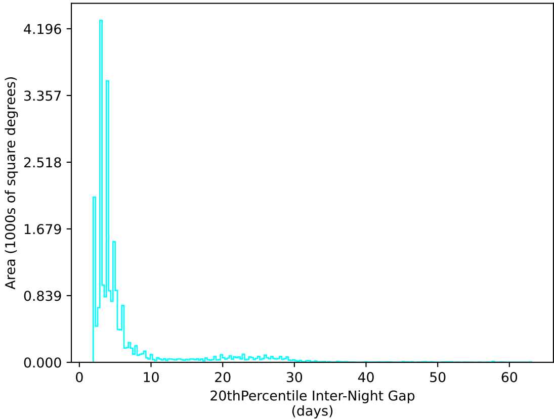
ddf_acor_sf20_ls40_lsr10_v3.4_10yrs All sky u band: 20thPercentile Inter-Night Gap
