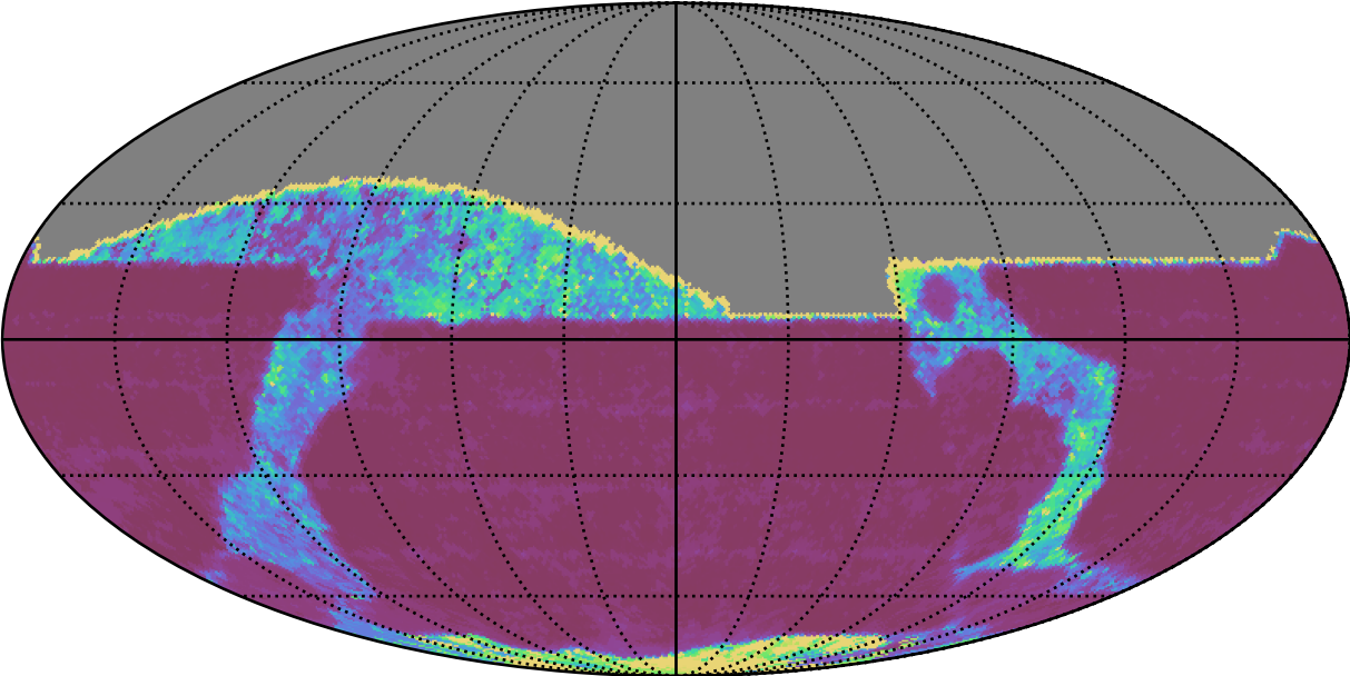
ddf_acor_sf20_lsf40_lsr10_v3.4_10yrs All sky i band: 20thPercentile Inter-Night Gap
