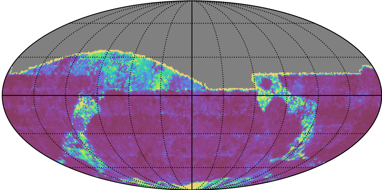
ddf_acor_sf20_lsf40_lsr10_v3.4_10yrs All sky g band: 20thPercentile Inter-Night Gap
