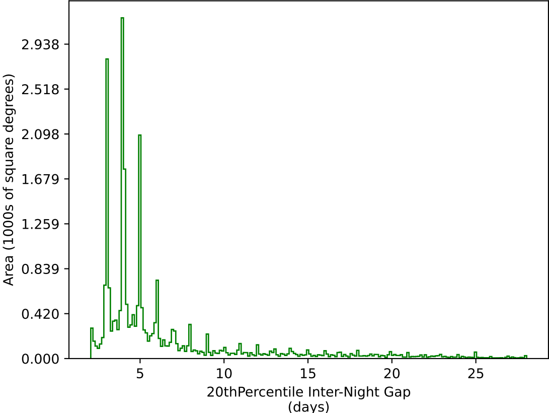
ddf_acor_sf20_lsf40_lsr10_v3.4_10yrs All sky g band: 20thPercentile Inter-Night Gap
