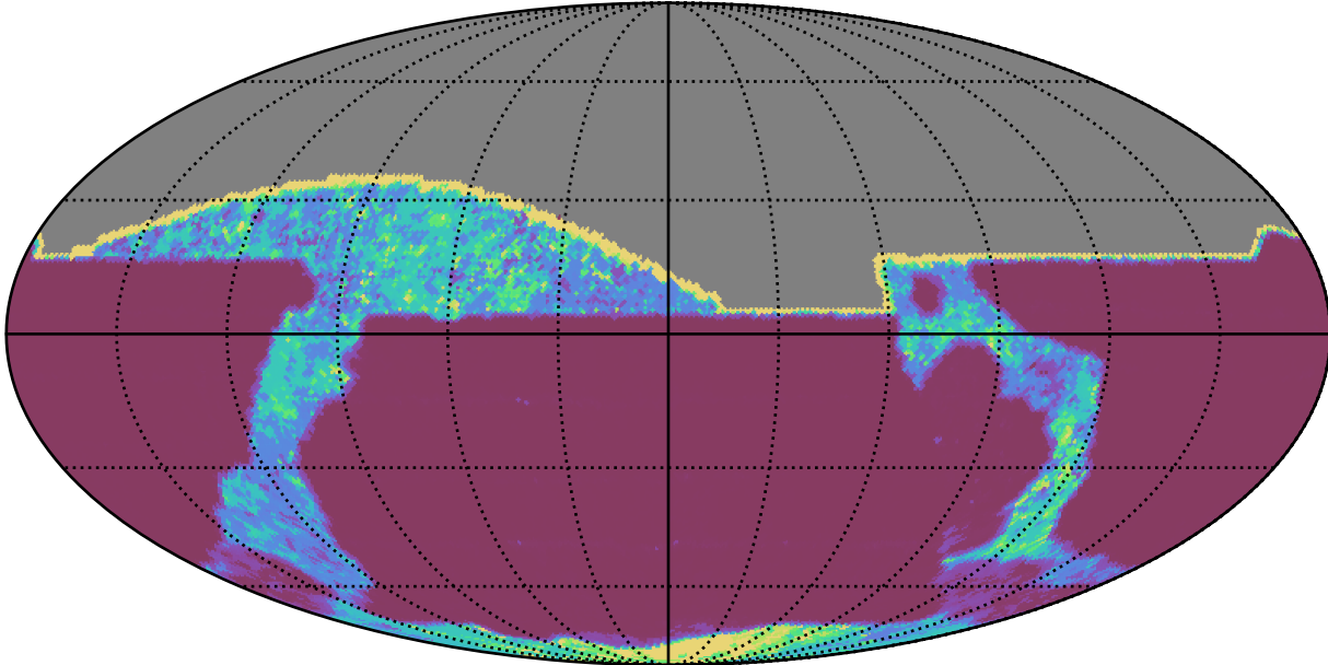
ddf_acor_sf20_lsf40_lsr10_v3.4_10yrs All sky all bands: 20thPercentile Inter-Night Gap
