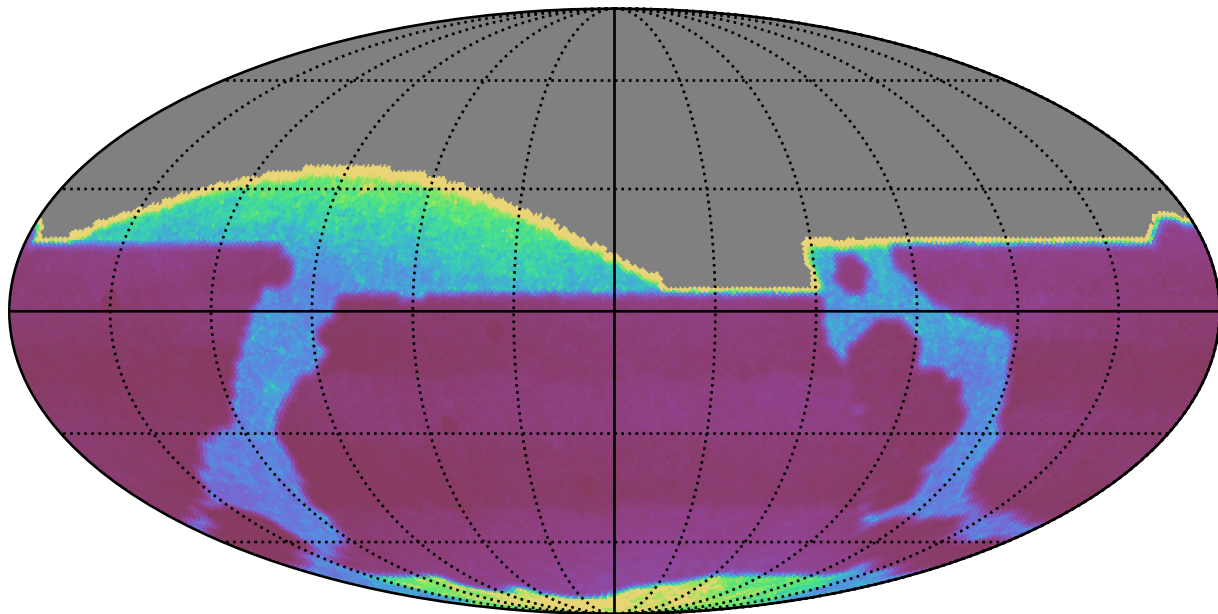
ddf_acor_sf20_lsf40_lsr10_v3.4_10yrs : properMotion
