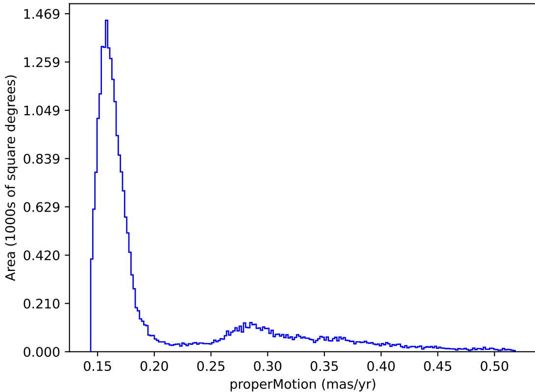
ddf_acor_sf20_lsf40_lsr10_v3.4_10yrs : properMotion
