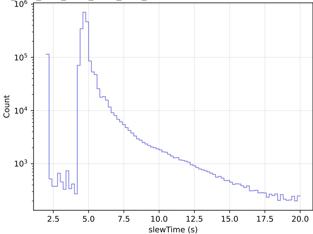
ddf_acor_sf20_Isf40_Isr10_v3.4_10yrs All visits: Zoom Slew Time Histogram
