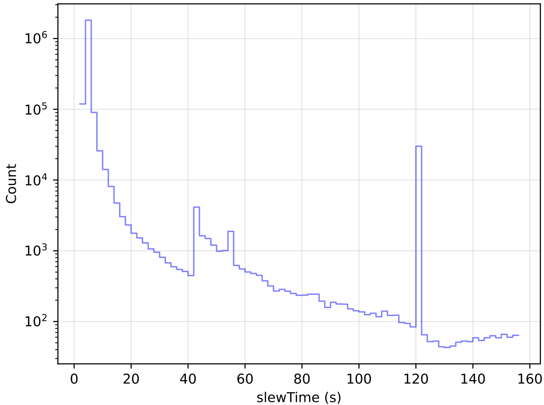
ddf_acor_sf20_lsf40_lsr10_v3.4_10yrs All visits: Slew Time Histogram
