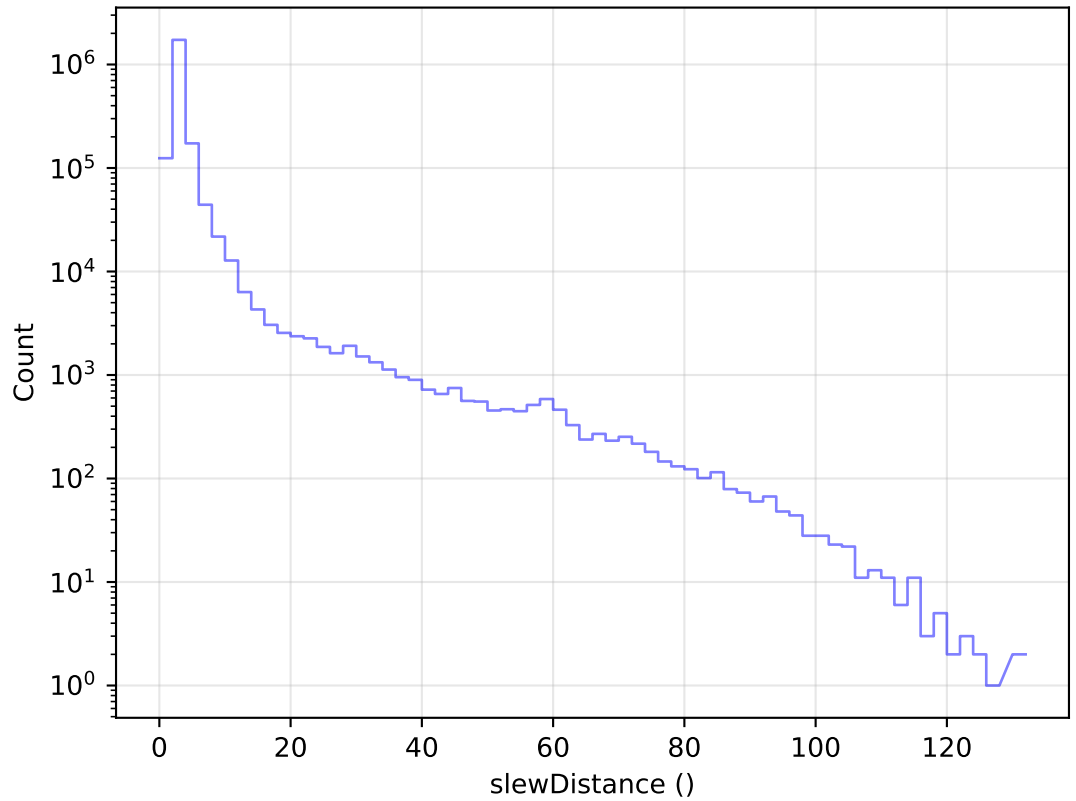
ddf_acor_sf20_lsf40_lsr10_v3.4_10yrs All visits: Slew Distance Histogram
