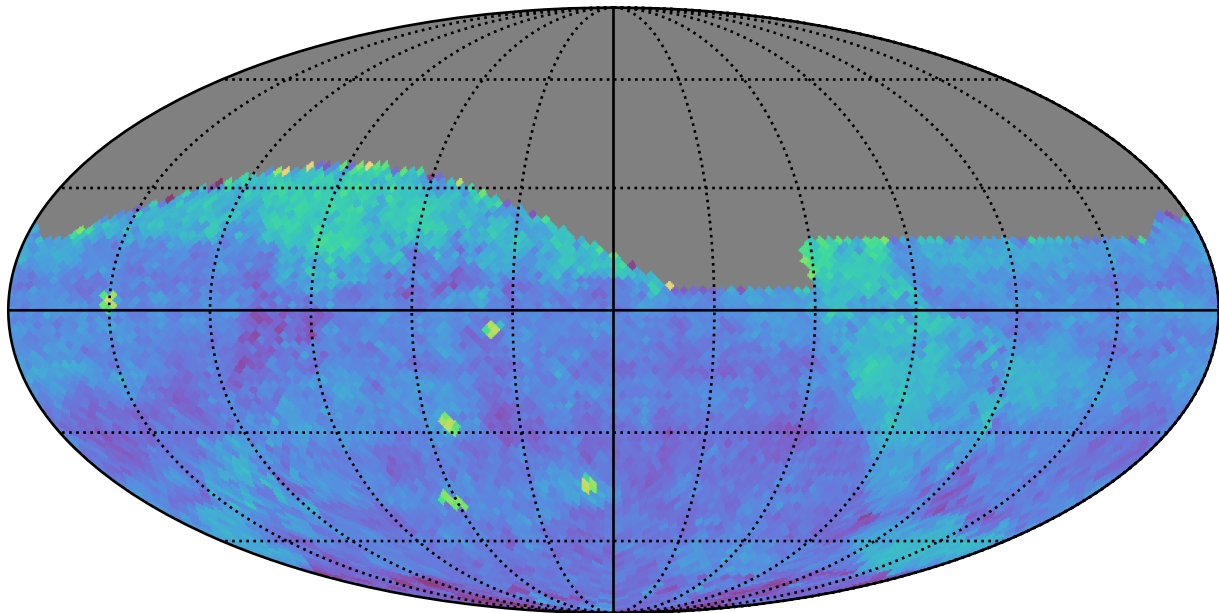
ddf_acor_sf20_lsf40_lsr10_v3.4_10yrs (g or r or i): PairFraction
