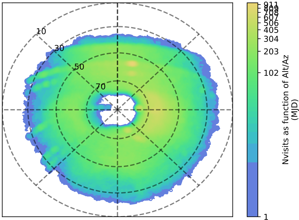
ddf_acor_sf20_ls40_lsr10_v3.4_10yrs u: Nvisits as function of Alt/Az
