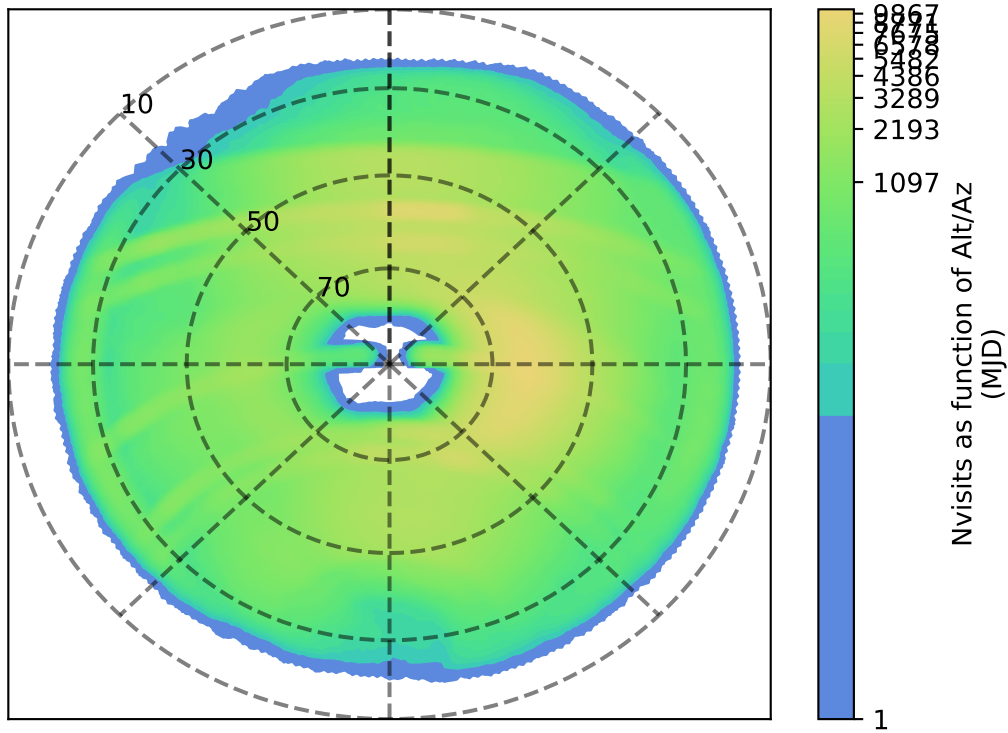
ddf_acor_sf20_lsf40_lsr10_v3.4_10yrs : Nvisits as function of Alt/Az
