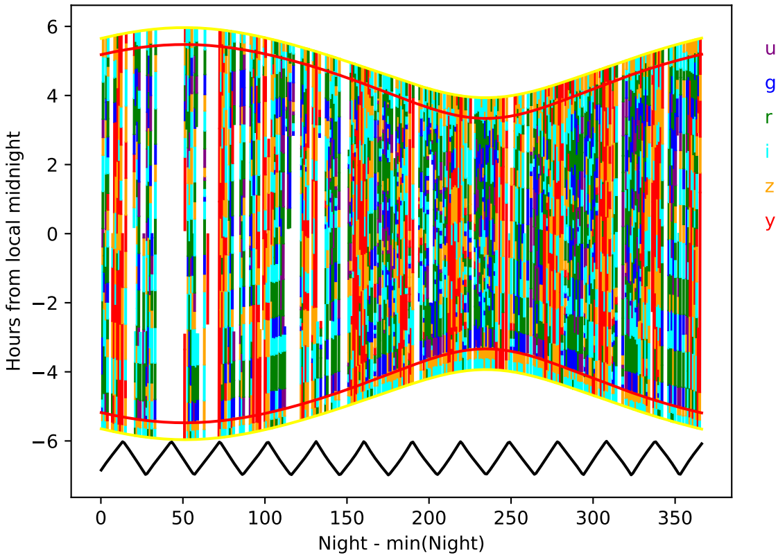
ddf_acor_sf20_ls40_lsr10_v3.4_10yrs year 8-9: Hourglass
