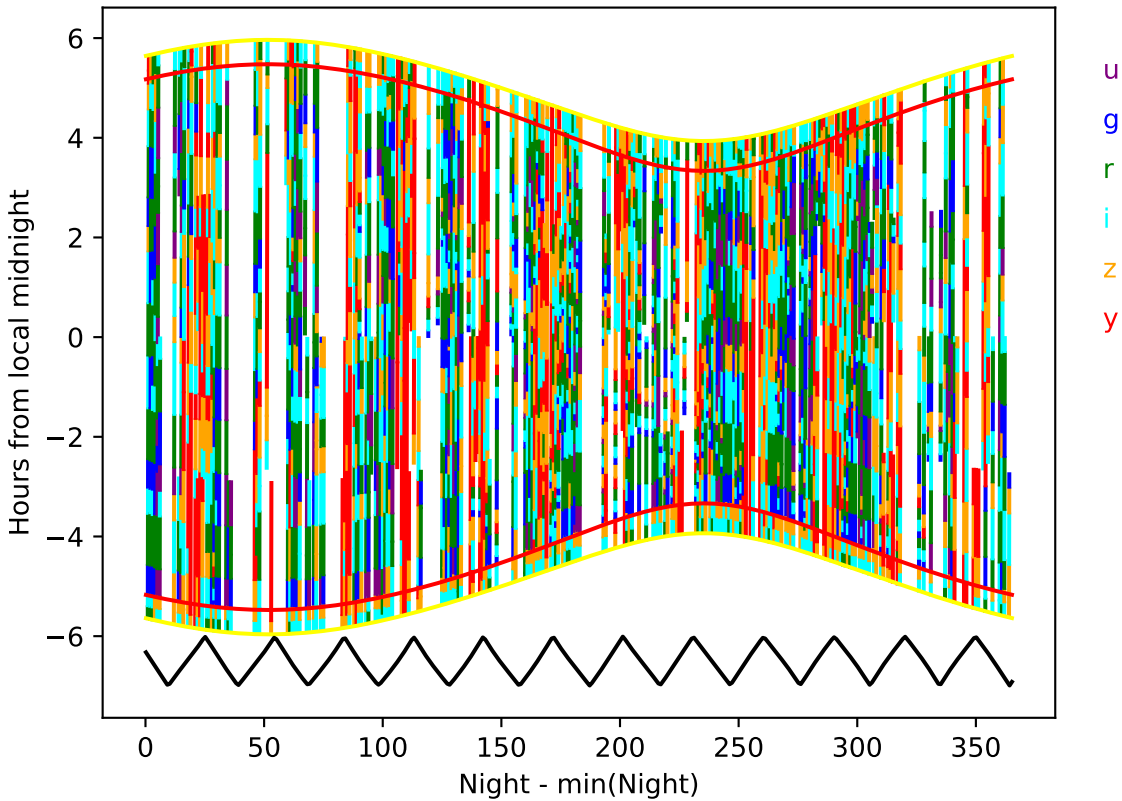
ddf_acor_sf20_lsf40_lsr10_v3.4_10yrs year 7-8: Hourglass
