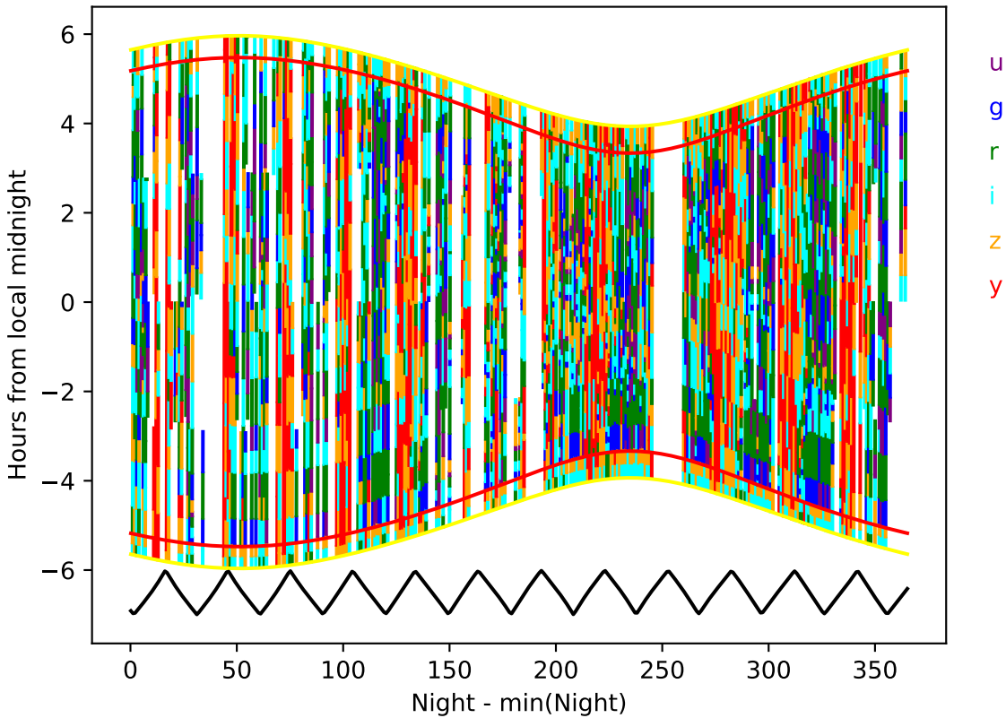
ddf_acor_sf20_ls40_lsr10_v3.4_10yrs year 5-6: Hourglass
