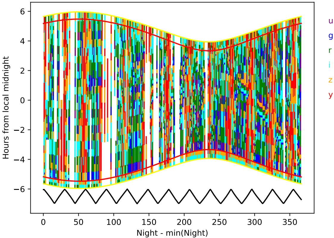
ddf_acor_sf20_lsf40_lsr10_v3.4_10yrs year 1-2: Hourglass
