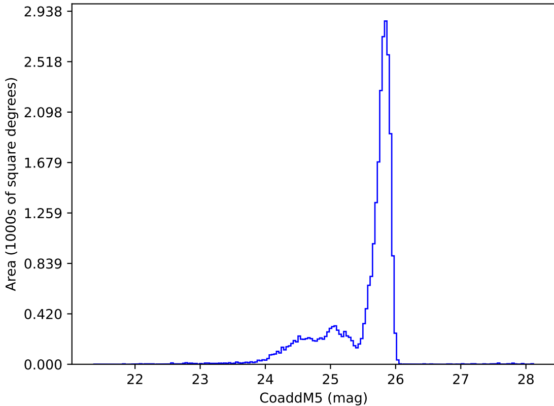
ddf_acor_sf20_lsf40_lsr10_v3.4_10yrs z: CoaddM5
