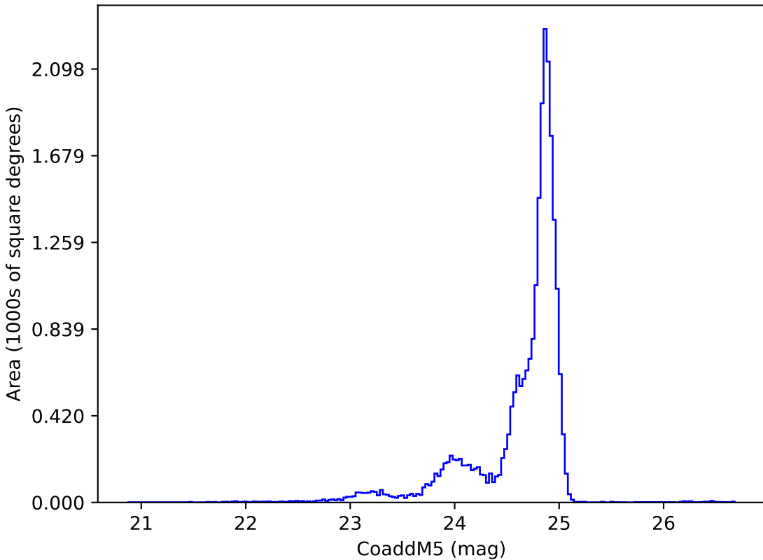
ddf_acor_sf20_lsf40_lsr10_v3.4_10yrs y: CoaddM5
