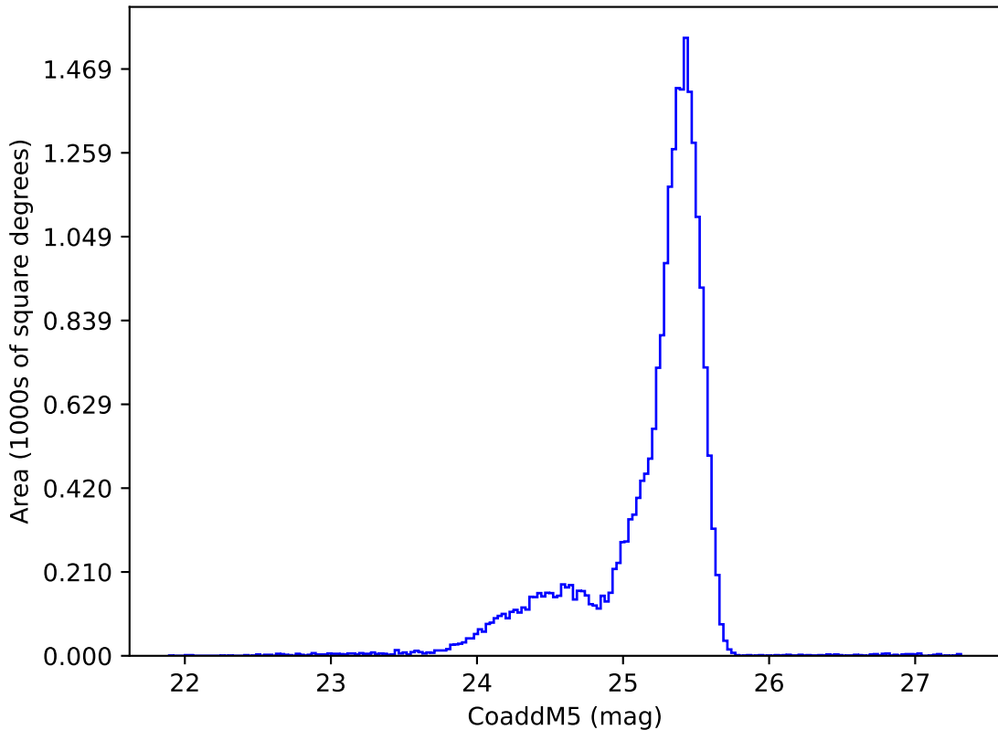
ddf_acor_sf20_lsf40_lsr10_v3.4_10yrs u: CoaddM5
