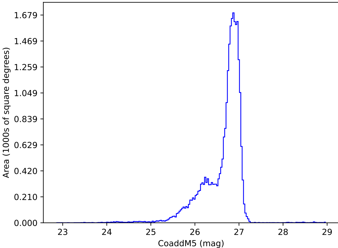
ddf_acor_sf20_lsf40_lsr10_v3.4_10yrs g: CoaddM5
