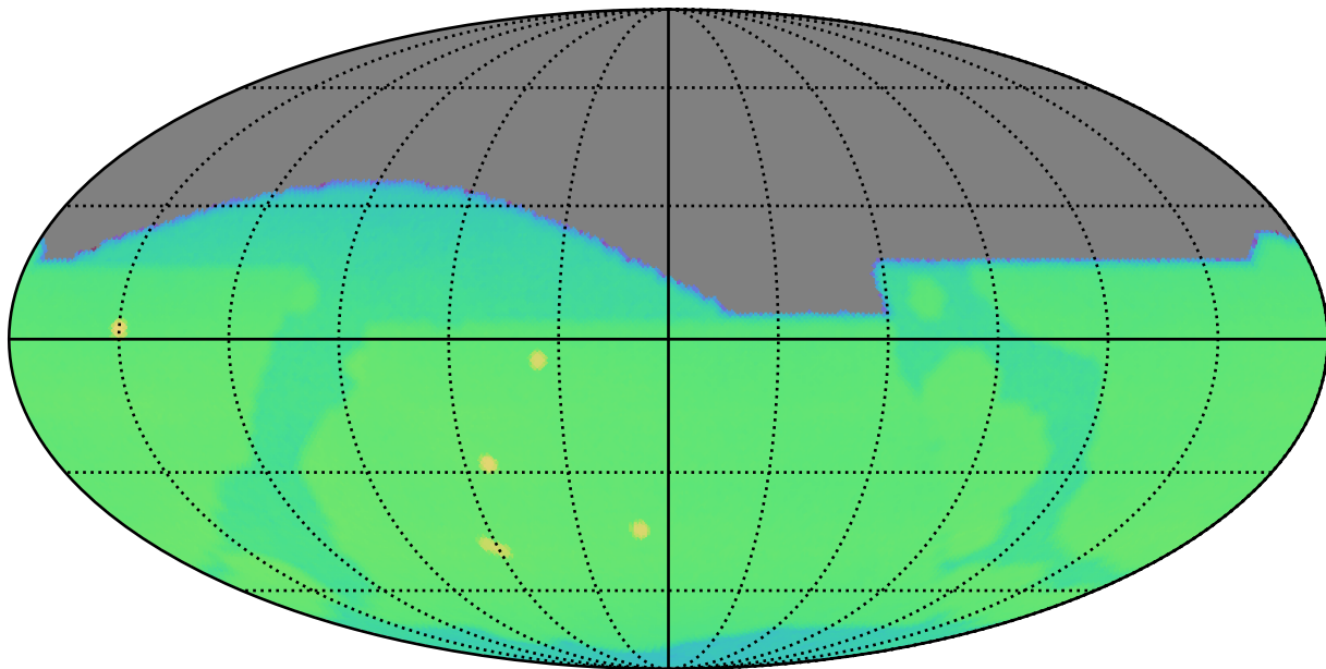
ddf_acor_sf20_lsf40_lsr10_v3.4_10yrs : CoaddM5
