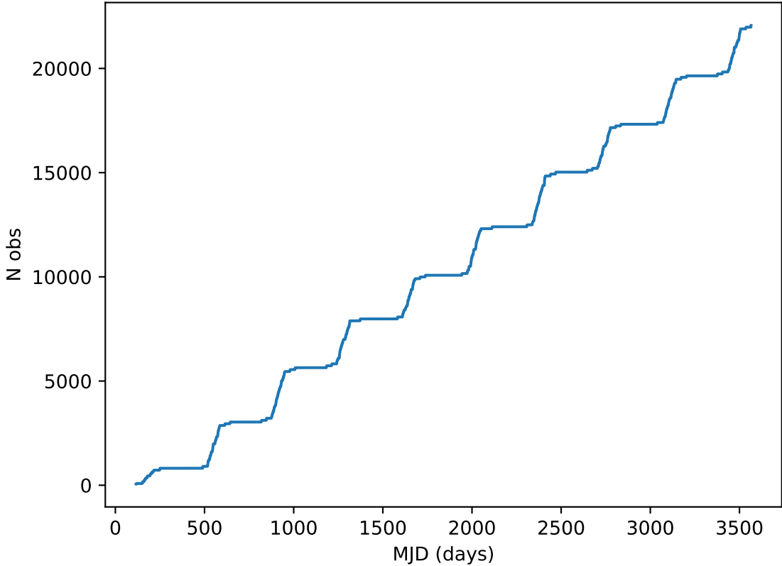
ddf_acor_sf20_lsf40_lsr10_v3.4_10yrs all bands: DD:XMM_LSS Cumulative NVisits
