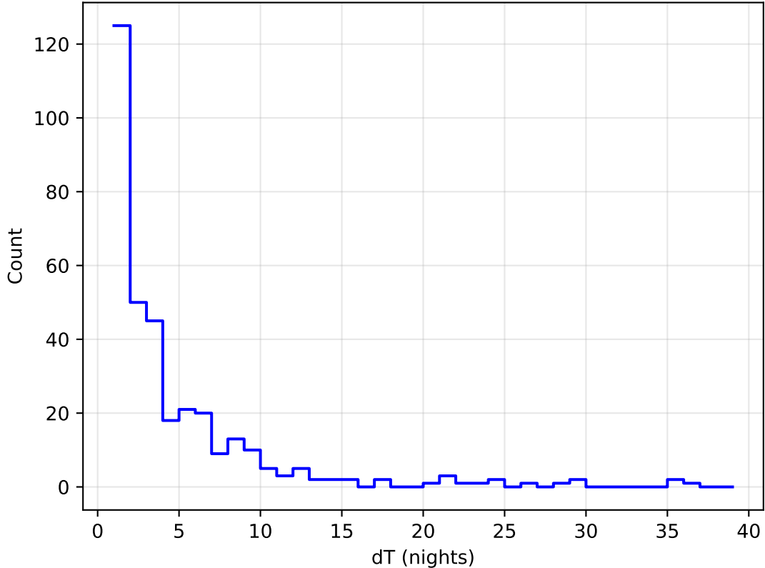
ddf_acor_sf20_lsf40_lsr10_v3.4_10yrs all bands: DD:WFD Delta Nights Histogram
