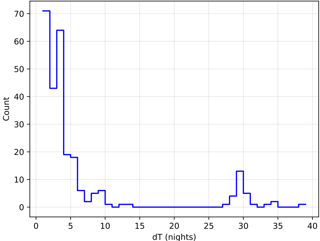
ddf_acor_sf20_lsf40_lsr10_v3.4_10yrs all bands: DD:ELAISS1 Delta Nights Histogram
