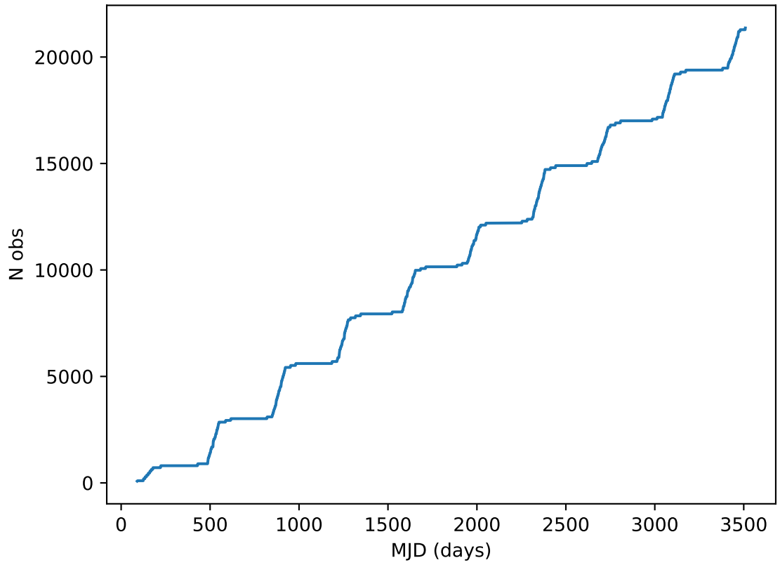
ddf_acor_sf20_lsf40_lsr10_v3.4_10yrs all bands: DD:ELAISS1 Cumulative NVisits
