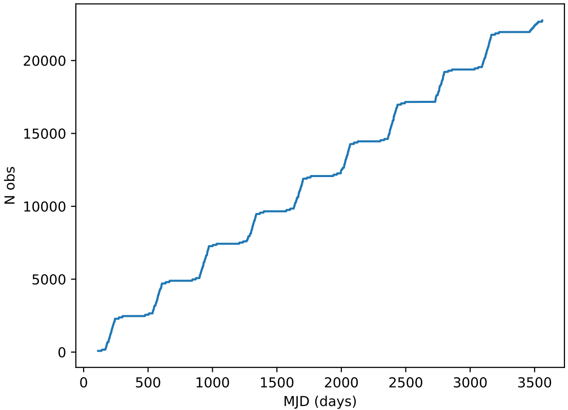
ddf_acor_sf20_lsf40_lsr10_v3.4_10yrs all bands: DD:EDFS Cumulative NVisits
