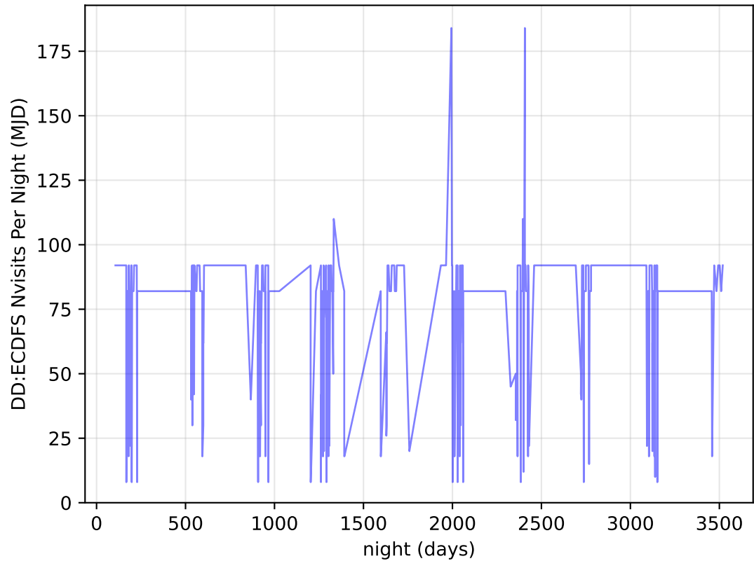
ddf_acor_sf20_lsf40_lsr10_v3.4_10yrs all bands: DD:ECDFS Nvisits Per Night
