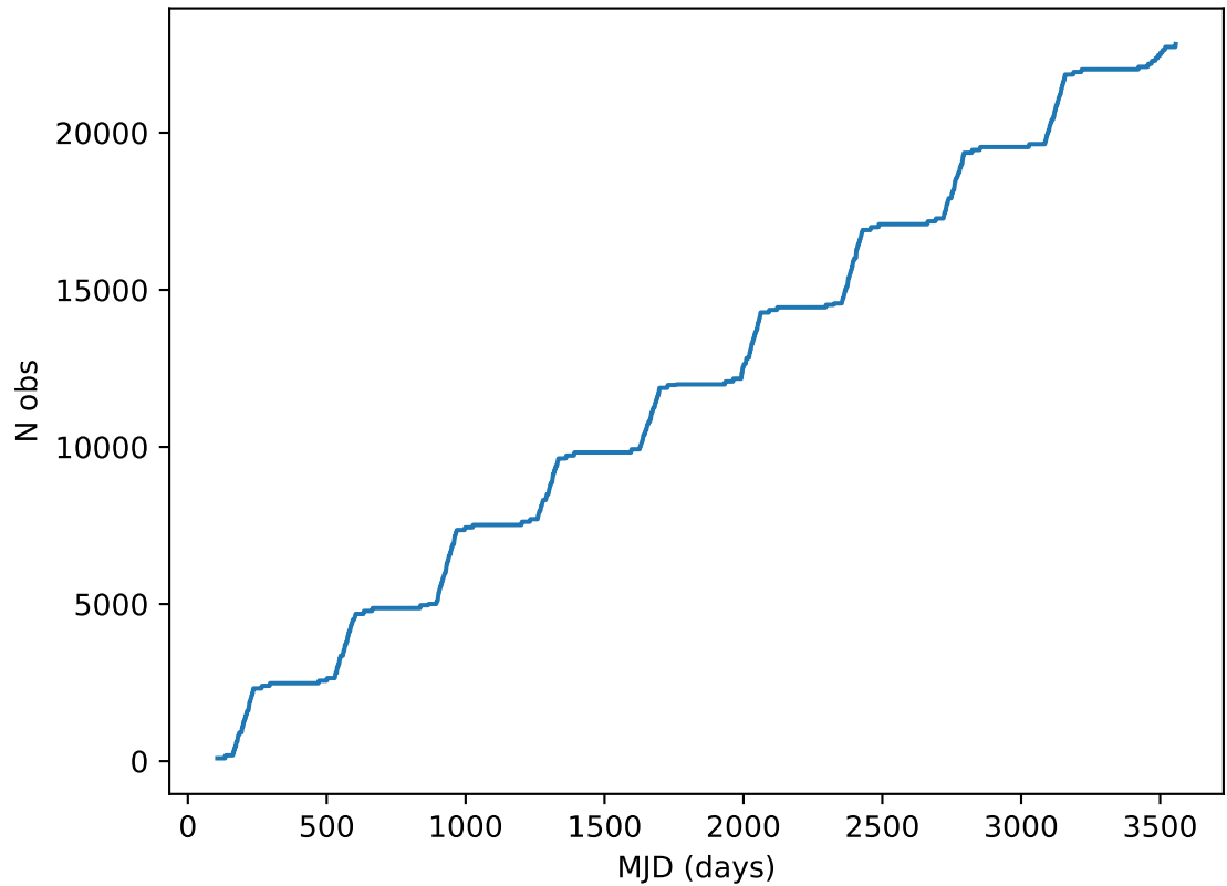
ddf_acor_sf20_lsf40_lsr10_v3.4_10yrs all bands: DD:ECDFS Cumulative NVisits
