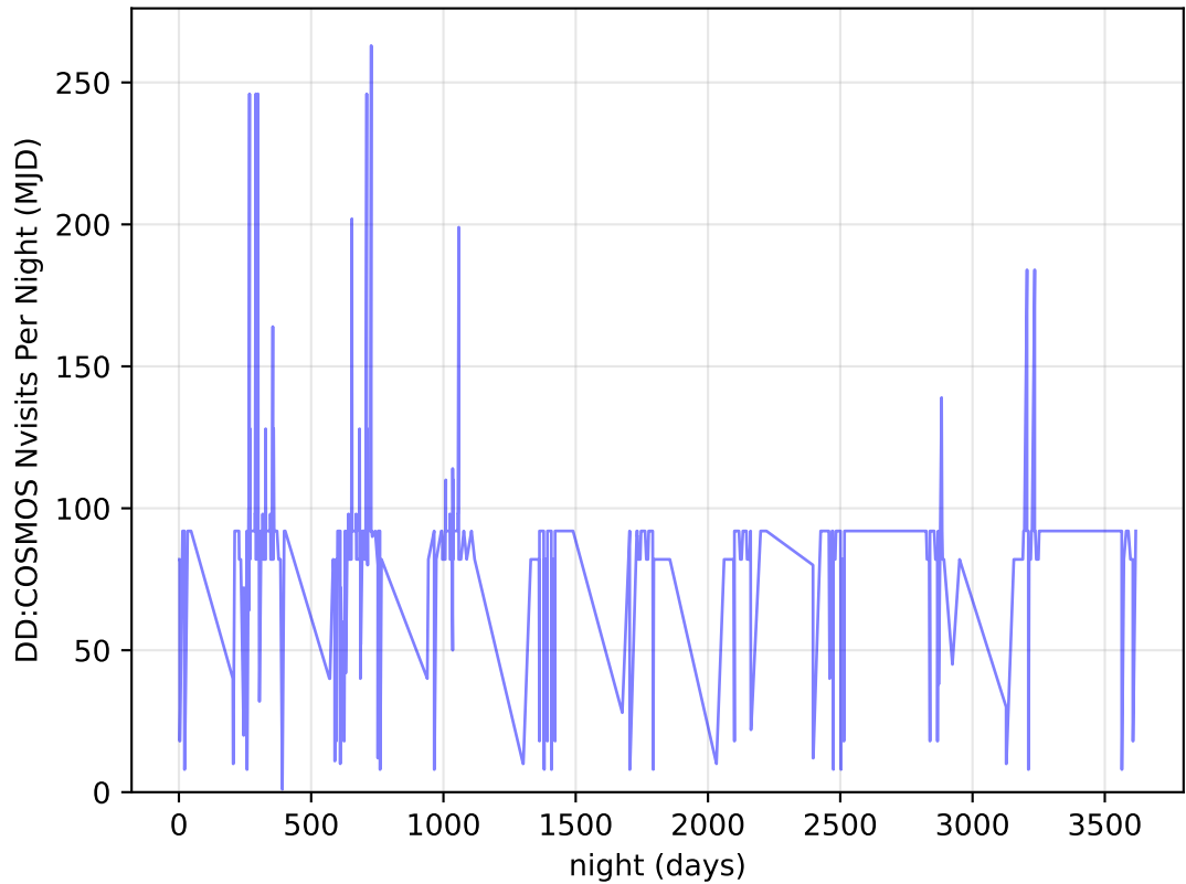
ddf_acor_sf20_lsf40_lsr10_v3.4_10yrs all bands: DD:COSMOS Nvisits Per Night
