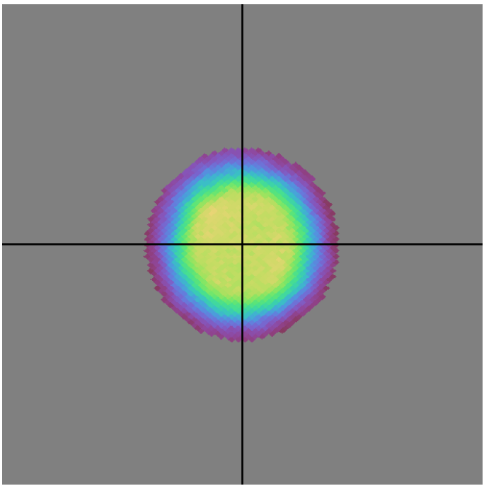
ddf_acor_sf20_lsf40_lsr10_v3.4_10yrs all bands: DD:COSMOS N Unique Nights
