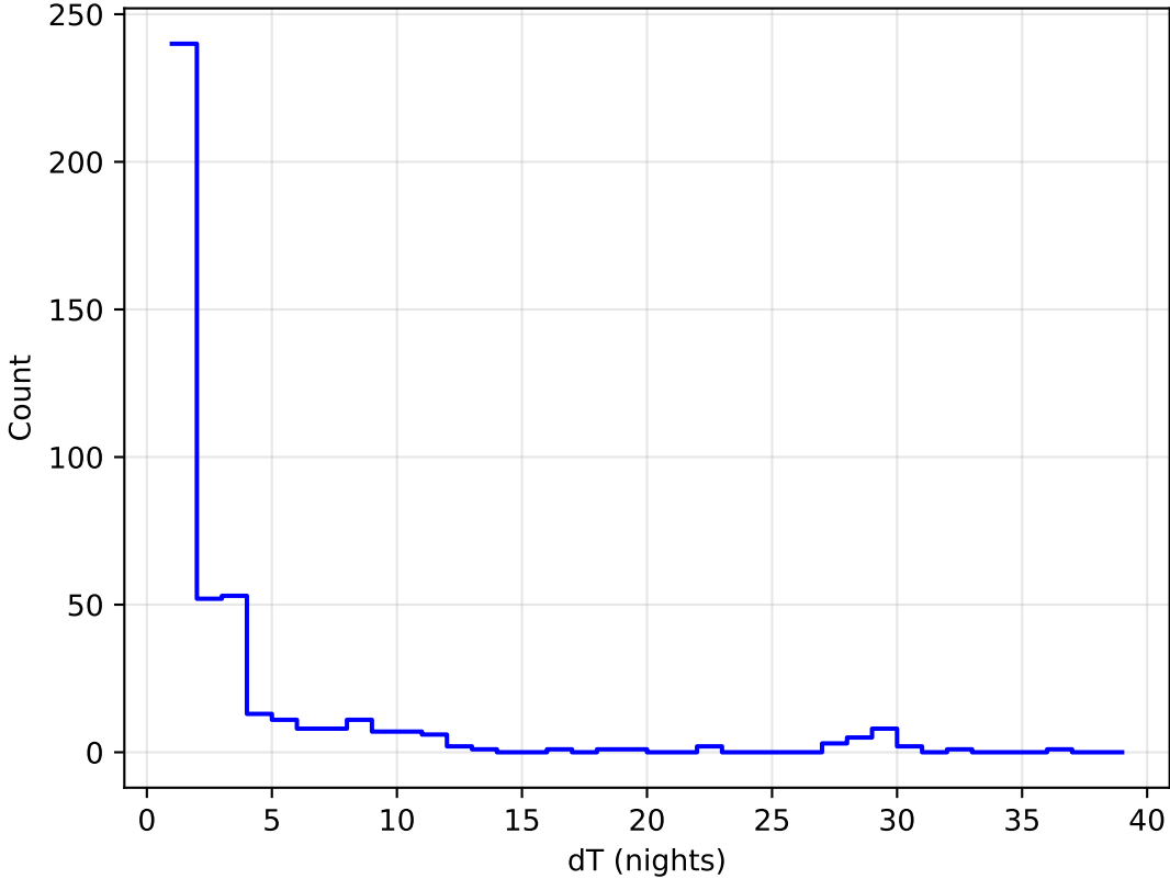
ddf_acor_sf20_Isf40_Isr10_v3.4_10yrs all bands: DD: COSMOS Delta Nights Histogram
