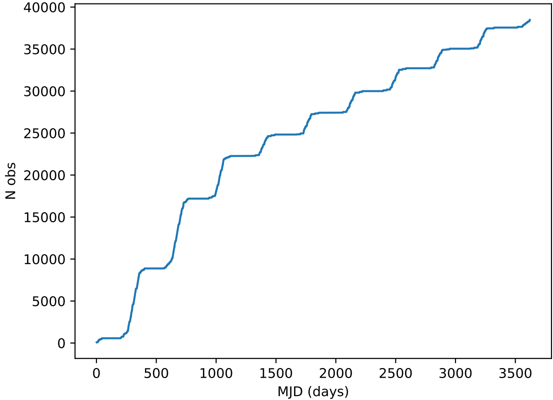
ddf_acor_sf20_lsf40_lsr10_v3.4_10yrs all bands: DD: COSMOS Cumulative NVisits
