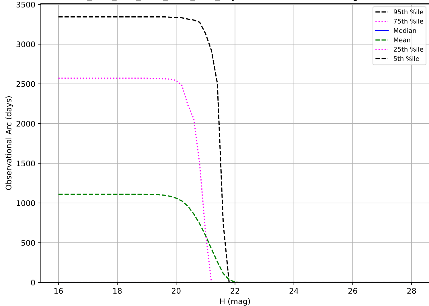
ddf_acor_sf20_lsf30_lsr50_v3.4_10yrs: Observational Arc Length Vatira
