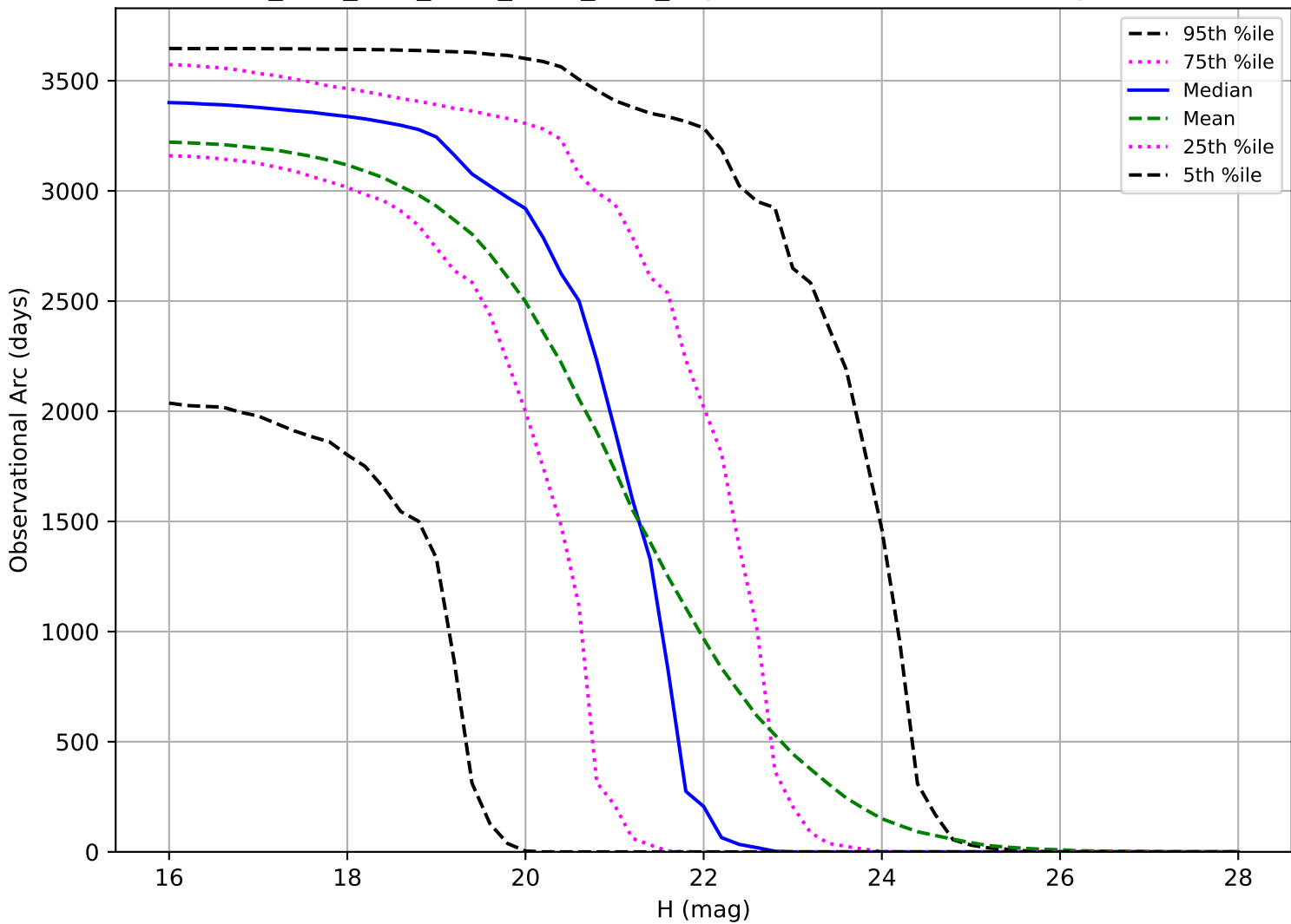
ddf_acor_sf20_lsf30_lsr50_v3.4_10yrs: Observational Arc Length PHA
