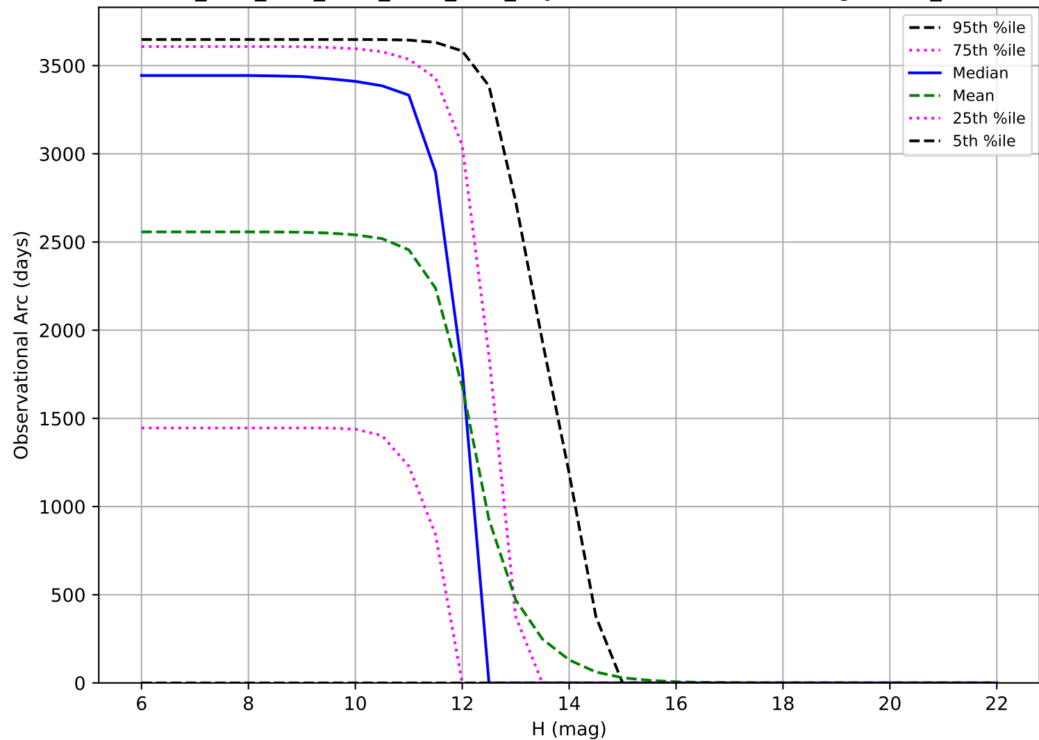
ddf_acor_sf20_lsf30_lsr50_v3.4_10yrs: Observational Arc Length OCC_r20
