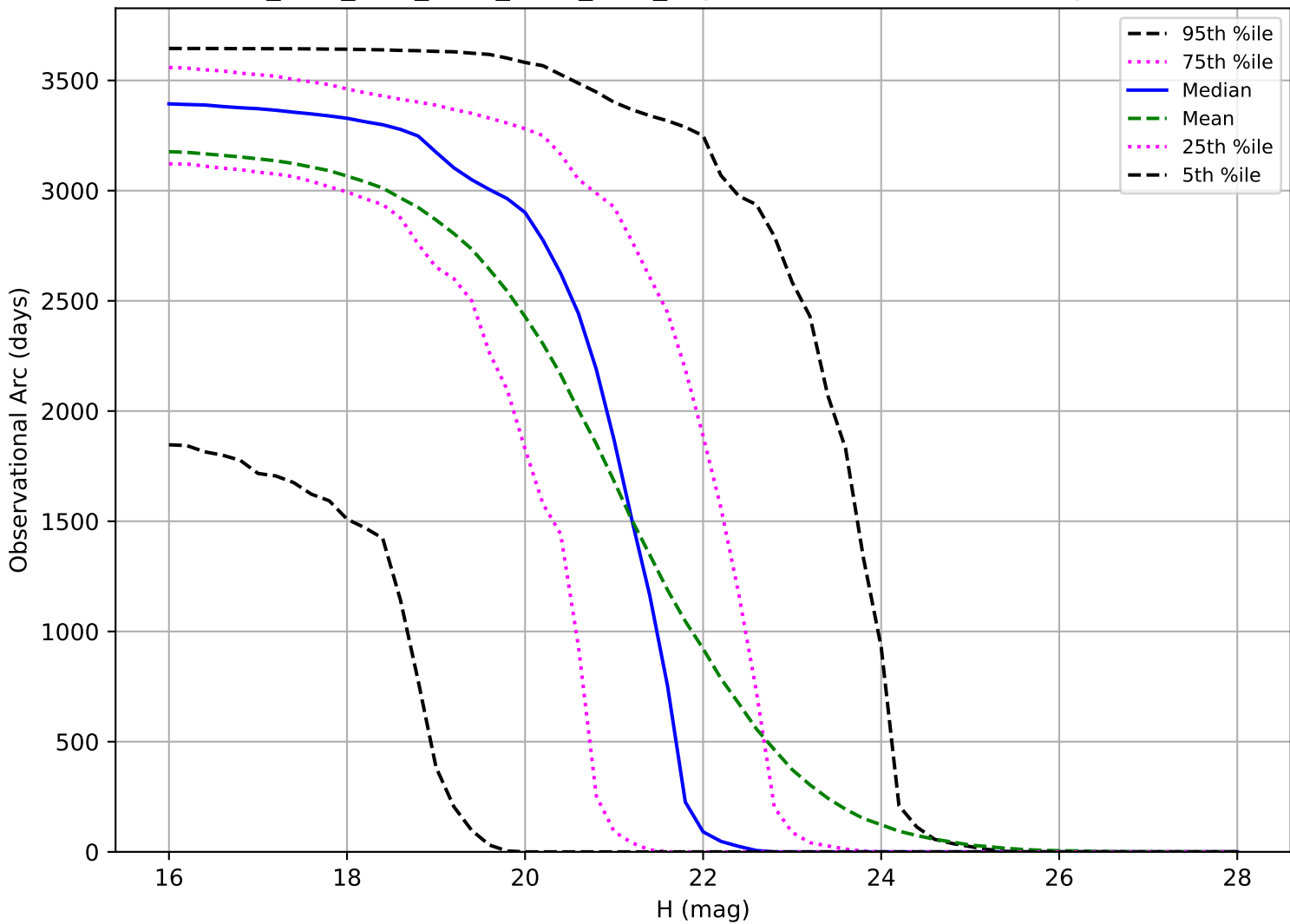
ddf_acor_sf20_lsf30_lsr50_v3.4_10yrs: Observational Arc Length NEO
