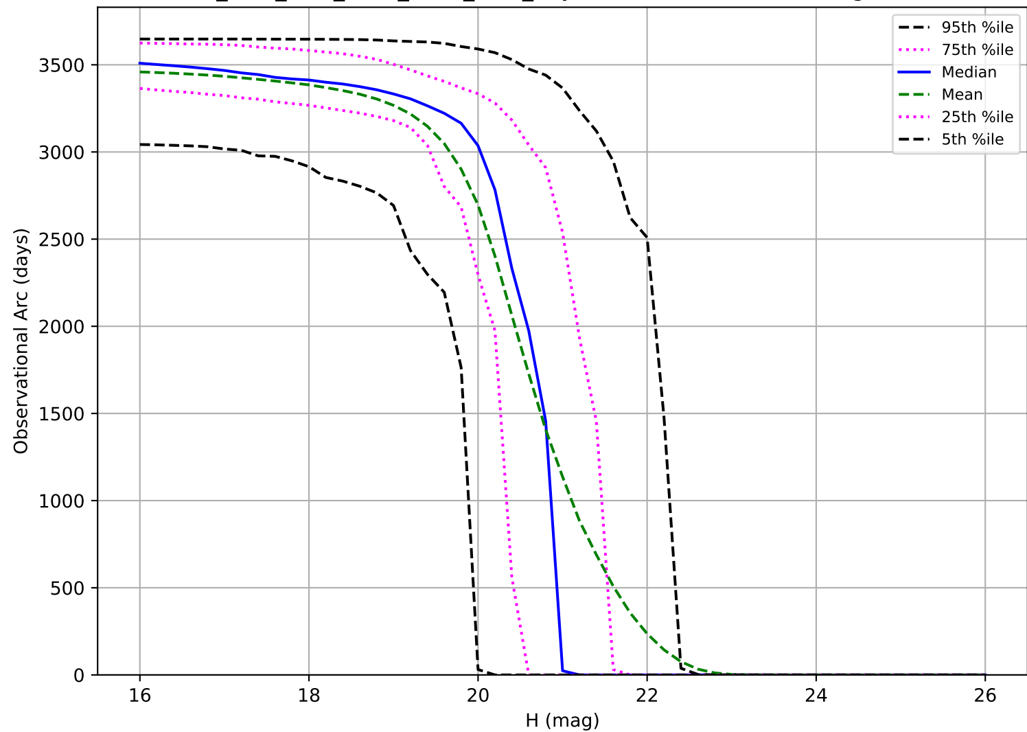
ddf_acor_sf20_lsf30_lsr50_v3.4_10yrs: Observational Arc Length MBA
