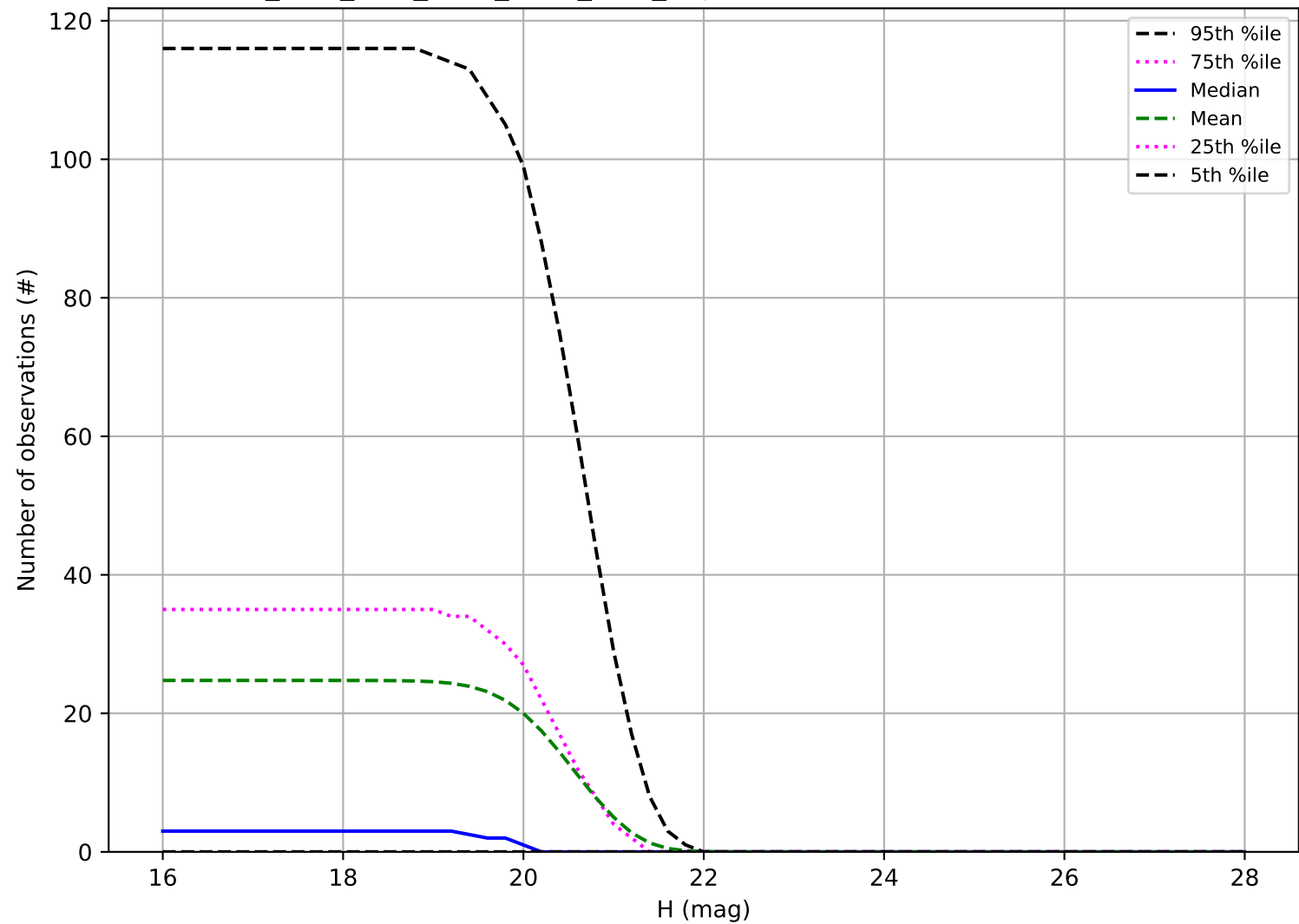
ddf_acor_sf20_lsf30_lsr50_v3.4_10yrs: Number of observations Vatira
