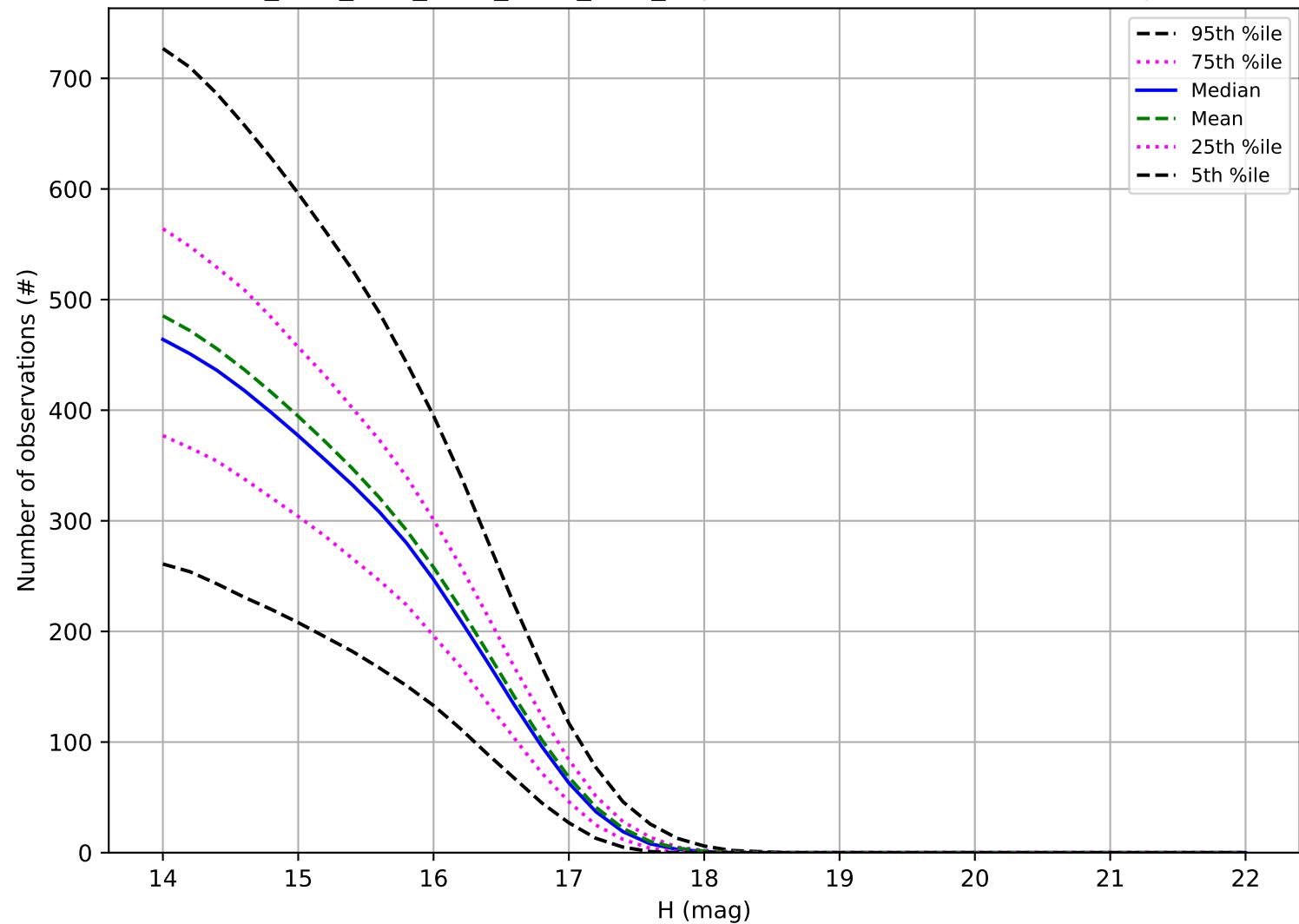
ddf_acor_sf20_lsf30_lsr50_v3.4_10yrs: Number of observations Trojan
