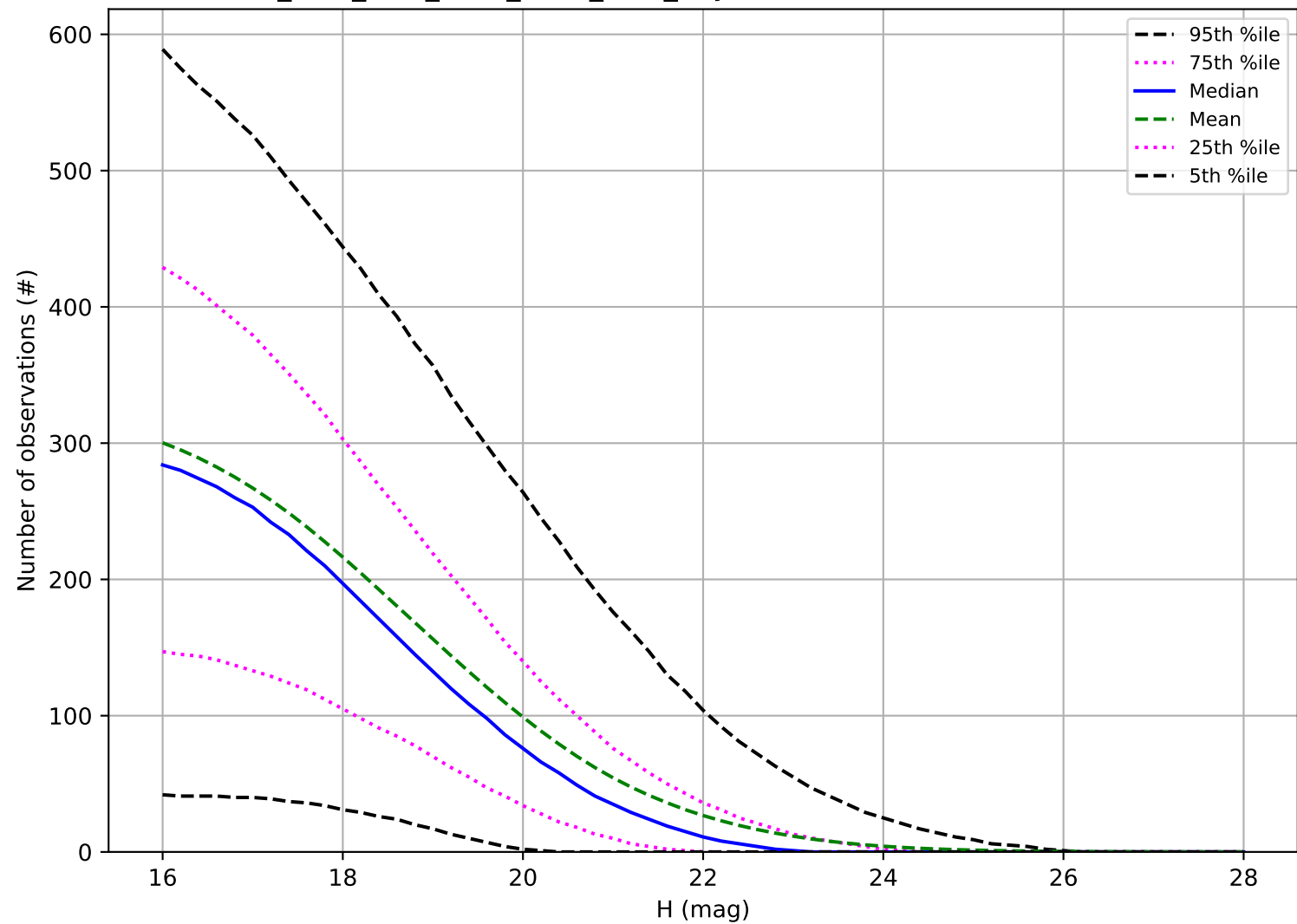
ddf_acor_sf20_lsf30_lsr50_v3.4_10yrs: Number of observations PHA
