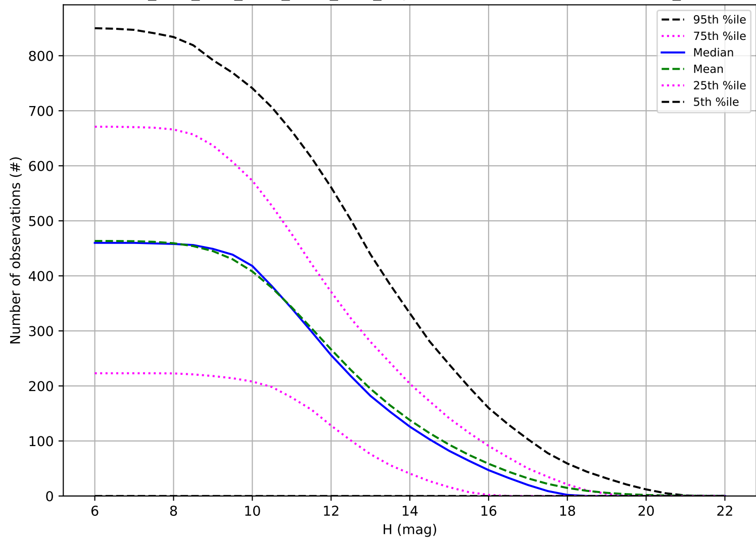
ddf_acor_sf20_lsf30_lsr50_v3.4_10yrs: Number of observations OCC_r5
