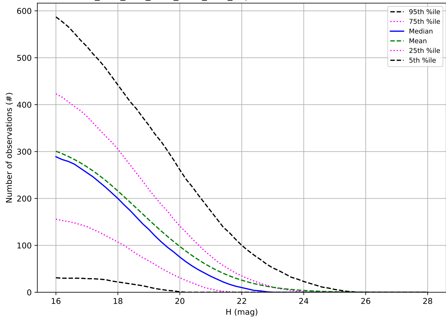
ddf_acor_sf20_lsf30_lsr50_v3.4_10yrs: Number of observations NEO
