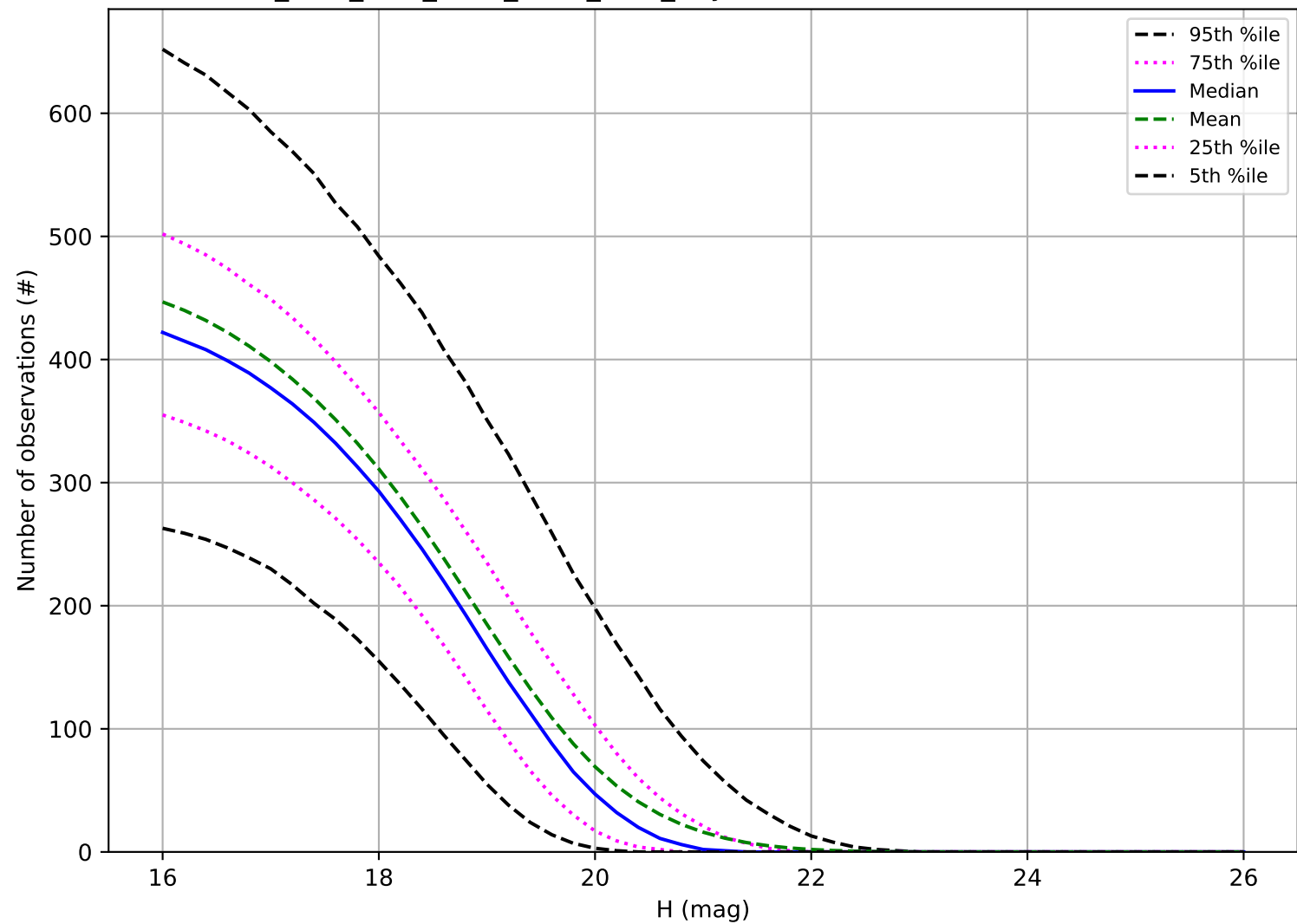
ddf_acor_sf20_lsf30_lsr50_v3.4_10yrs: Number of observations MBA
