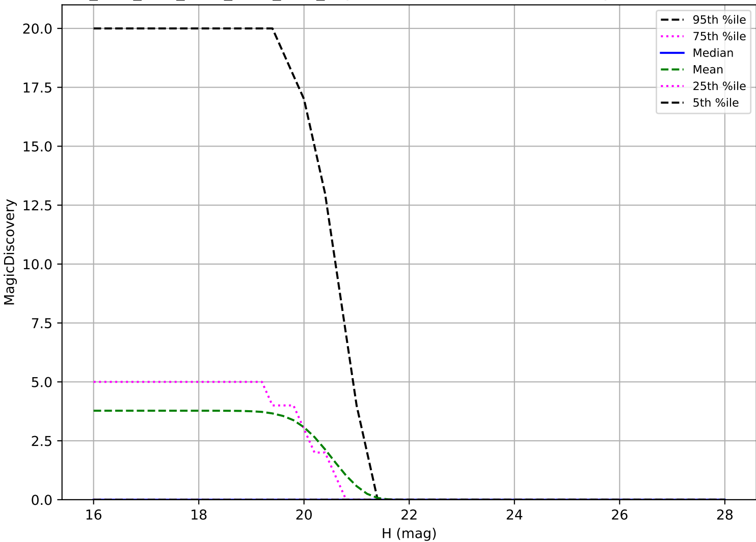
ddf_acor_sf20_lsf30_lsr50_v3.4_10yrs: Vatira 6 detections in 60 nights detection loss
